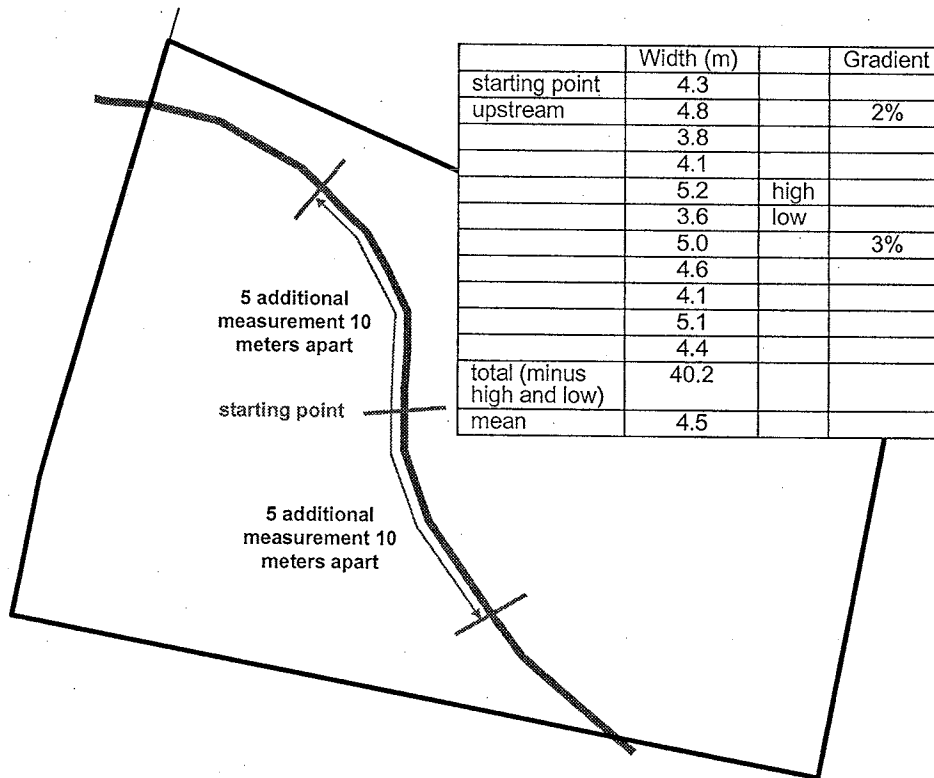
Figure 3-3: Calculating average channel width and channel slope
