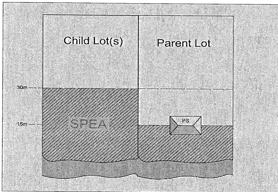
Figure 2-4 Example of Wide Lot Scenario. The SPEA is reduced on the Parent Lot where the Permanent Structure will remain but all Child lots where there are no permanent structures have the maximum SPEA width for their Vegetation Category/Fish Bearing Status.
